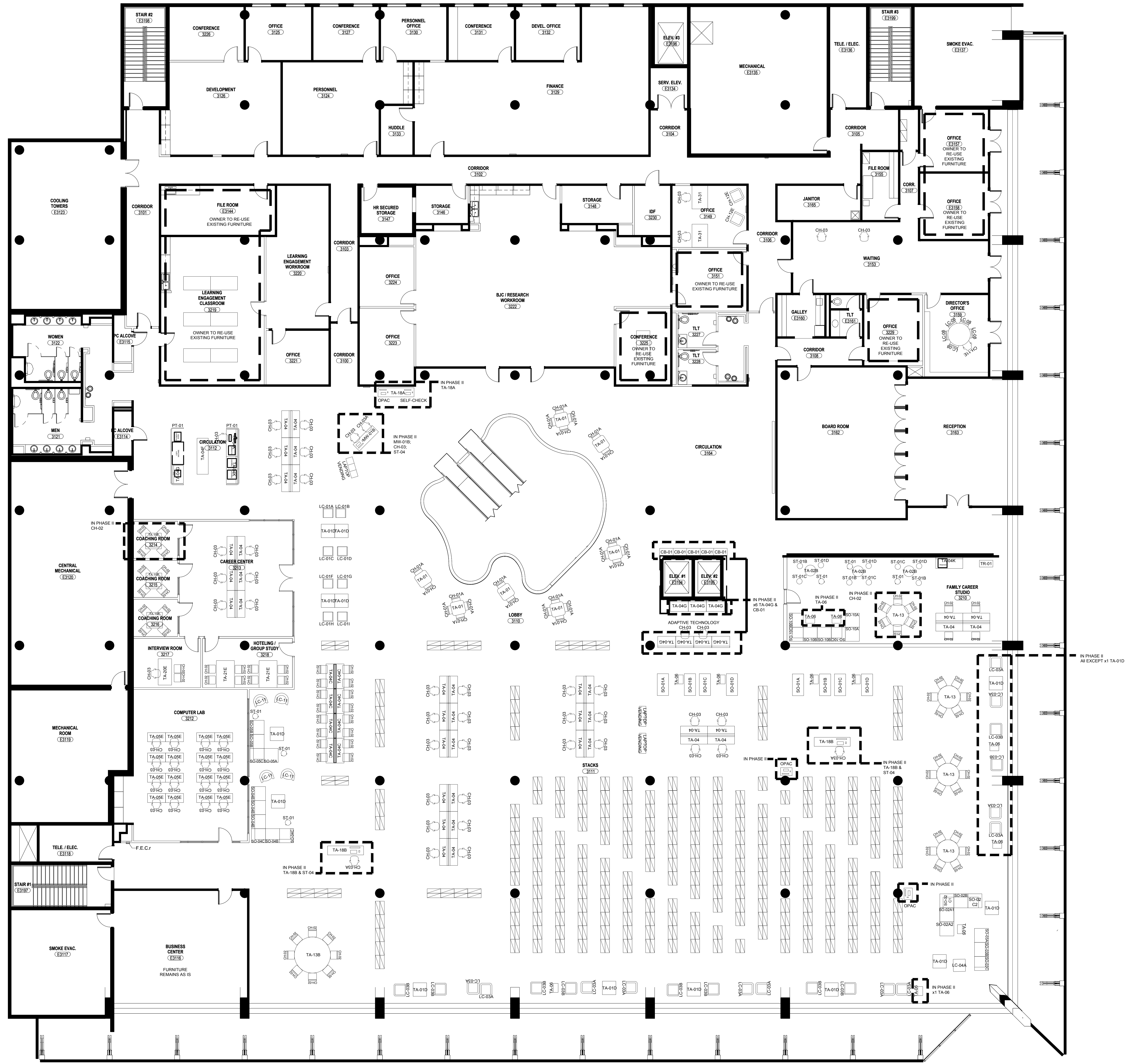
1 THIRD LEVEL FURNITURE PLAN 1/8" = 1'-0"
