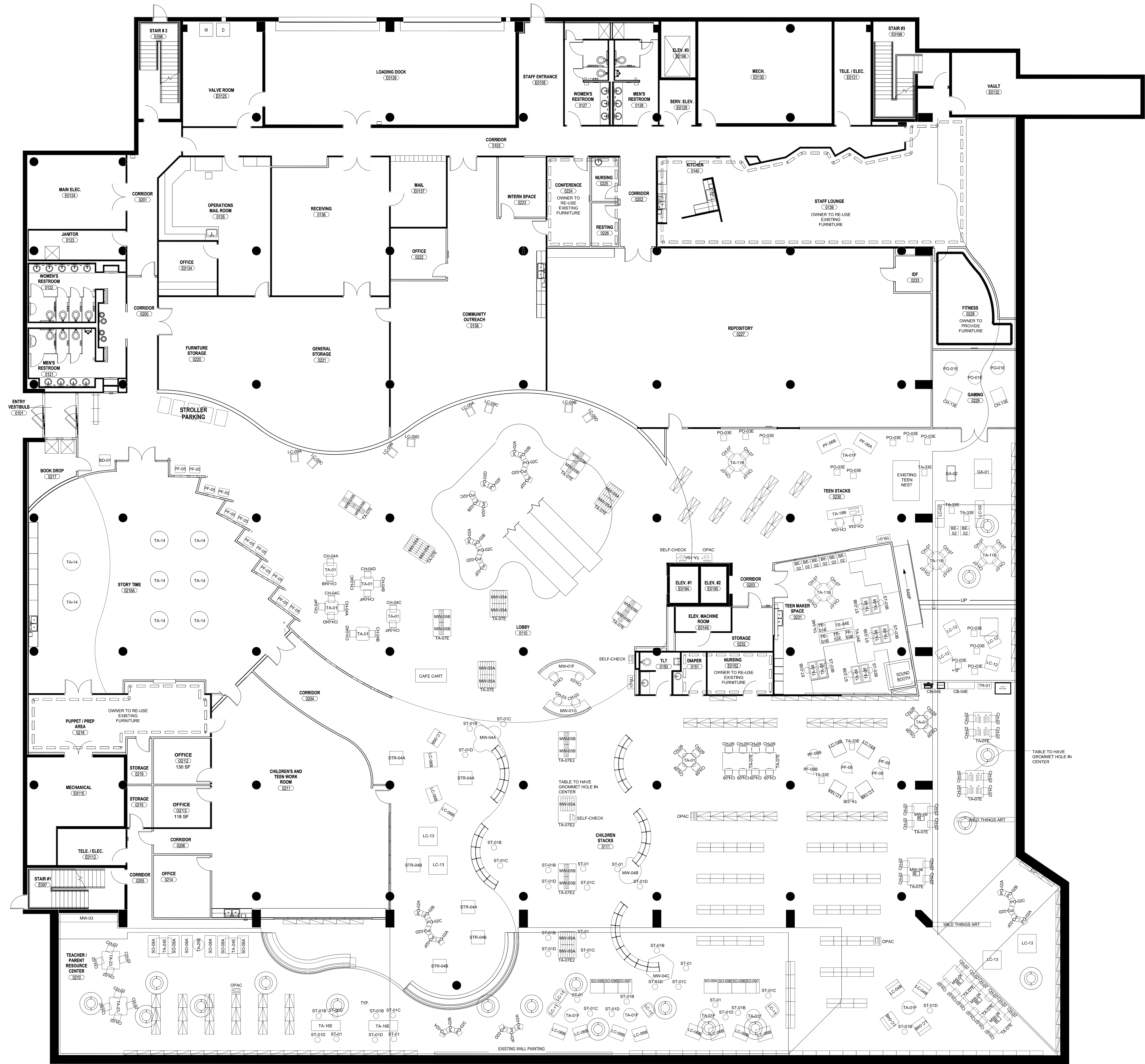
1 GARDEN LEVEL FURNITURE PLAN F1.0 1/8" = 1'-0"
